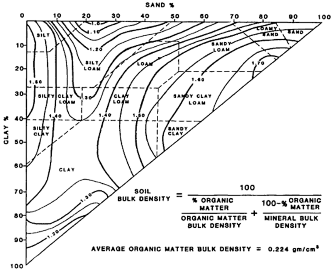
Figure 1. Mineral bulk density (g/cm 3 ).
